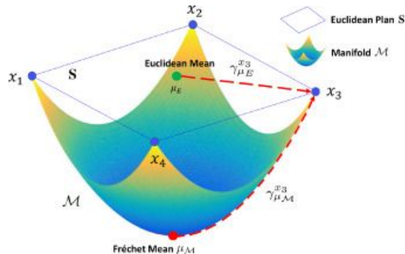
Fig 4. Frechet Mean Prompt Mixing
